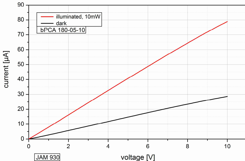
current-voltage characteristics
